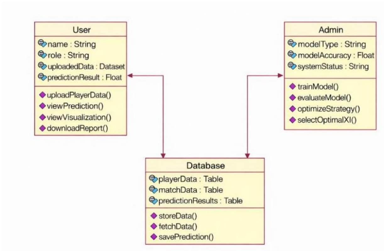
Fig 3.2: Class Diagram
