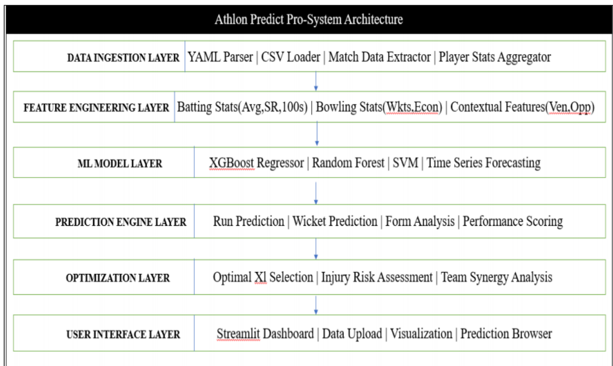
Fig 3.1: System Architecture
