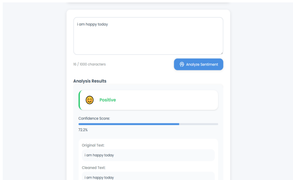
Fig 4: Analysis Result
