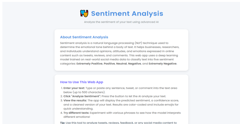
Fig 3:Sentiment Analysis
